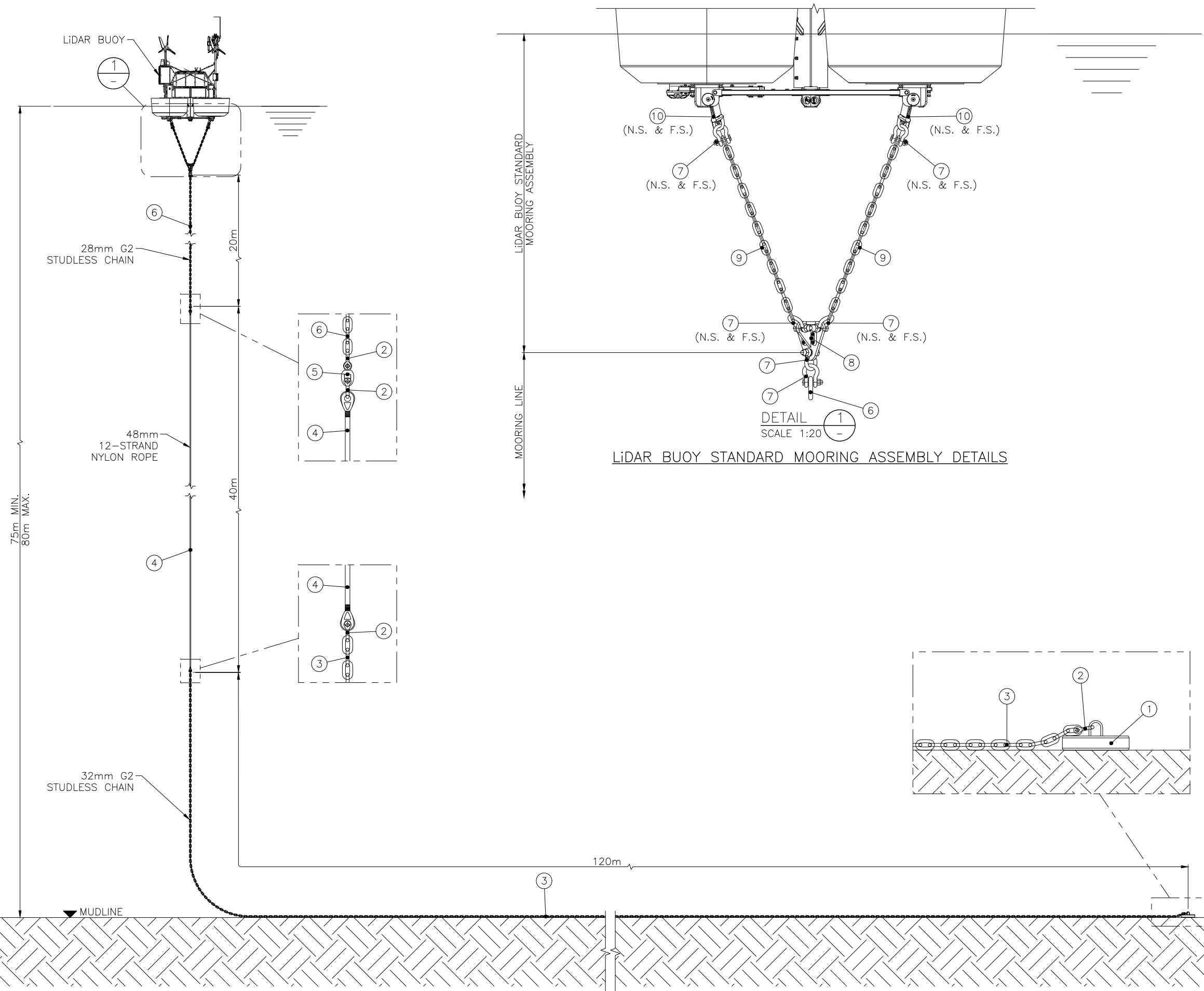
MOORING LINE MAKE UP ELEVATION – TEMPORARY SITE
