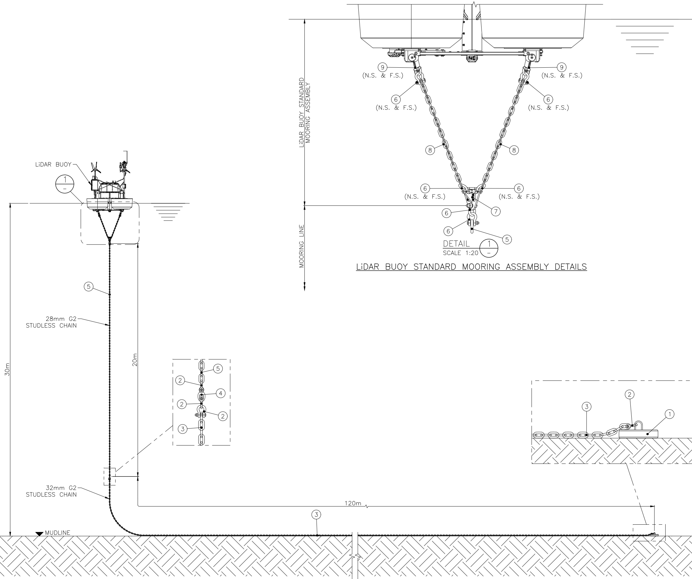
MOORING LINE MAKE UP ELEVATION – FINAL SITE
